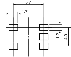
(Unit: mm)
