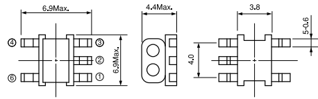
(Unit: mm)
