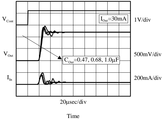
■ On/Off Transient ( V_{Cont}=0 \rightarrow 1.2V ) (TK68128AMF/M5/S2)
