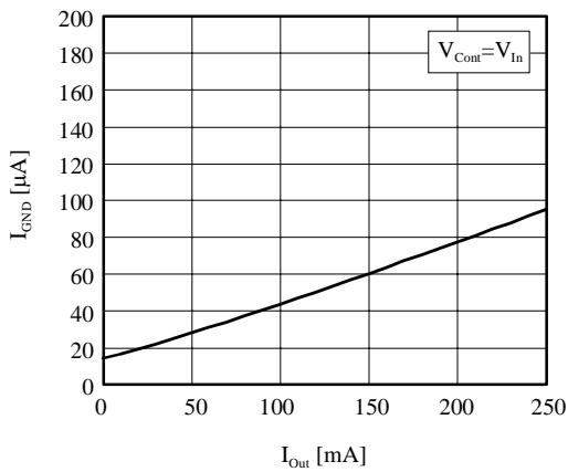
■ I_{GND} vs I_{Out} (TK68128AMF/M5/S2)
