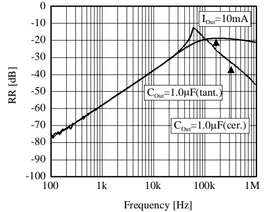
■ RR vs Frequency (TK68112AMF/M5/S2)
