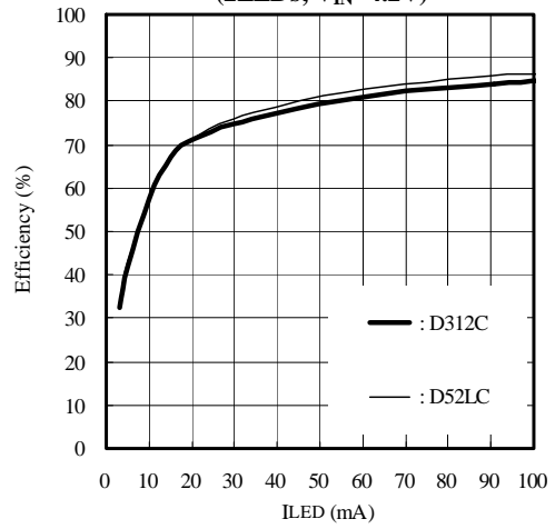
Efficiency vs. ILED (3LEDs, V IN =4.2V)
