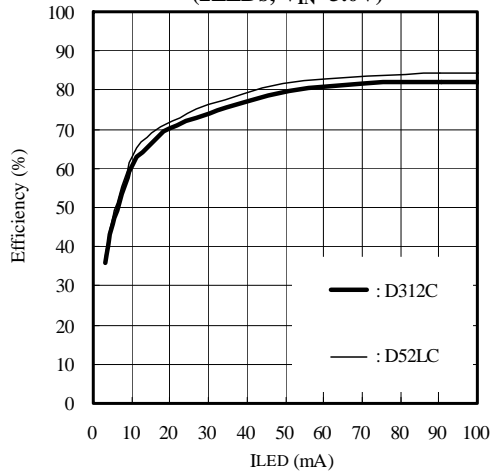
Efficiency vs. ILED (3LEDs, V IN =3.0V)
