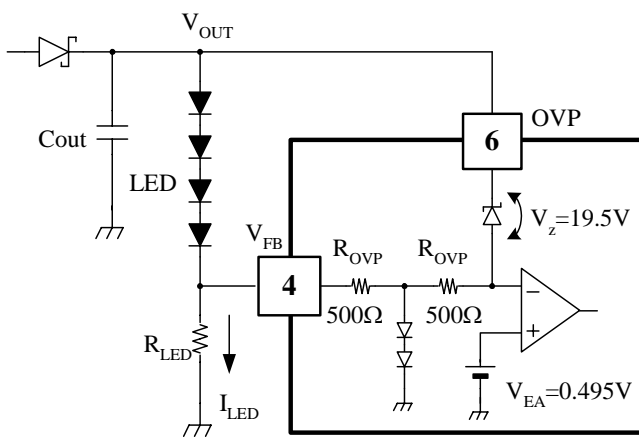
Fig3: Setting constant current through LED
