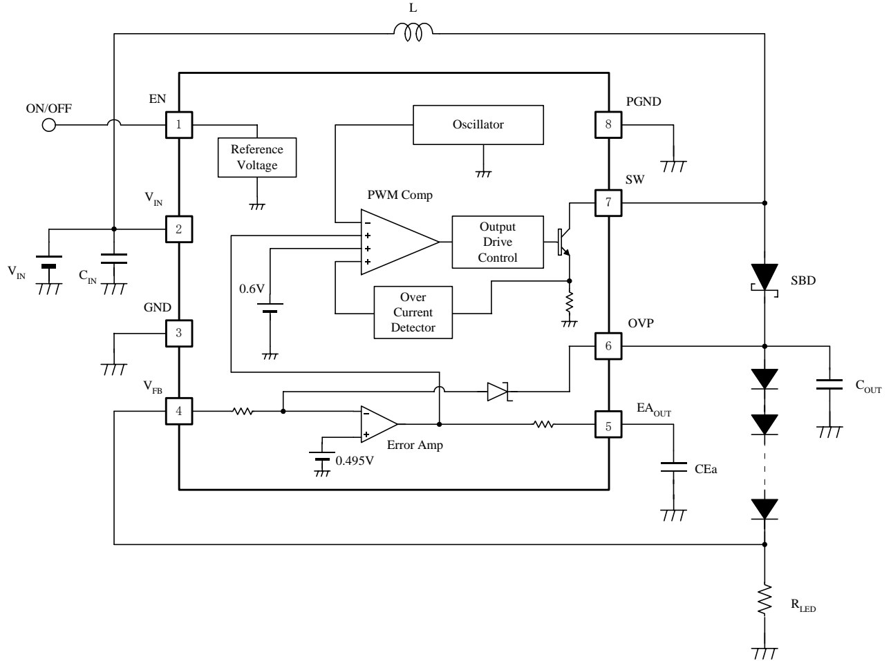
Fig.7: Typical 2-4 LEDs Application
