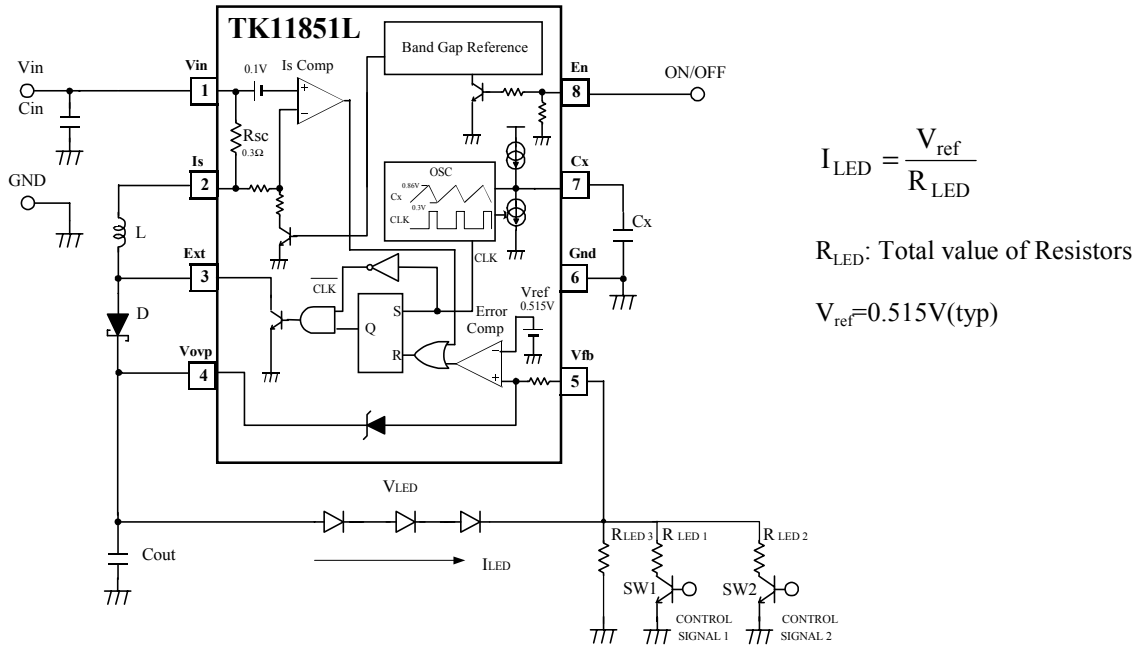
Figure 11: Example of 3LEDs with a 4 brightness level circuit
