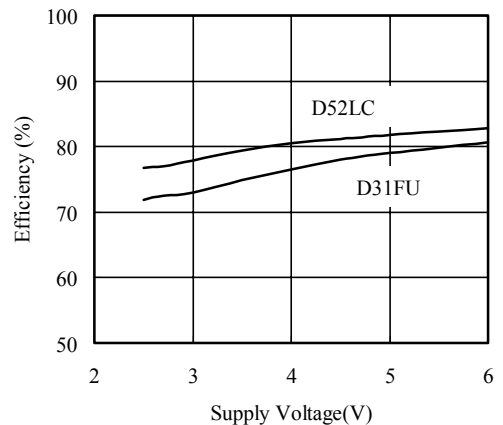
Efficiency vs. Supply Voltage
