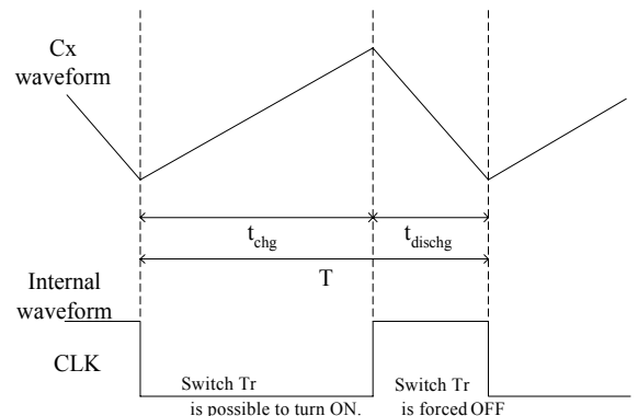
Figure 1: OSC Waveforms
