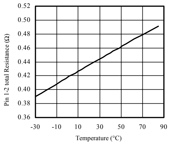
Pin 1-2 total Resistance vs. Temperature (V_{in}-V_{is})/I_L, I_L=100mA
